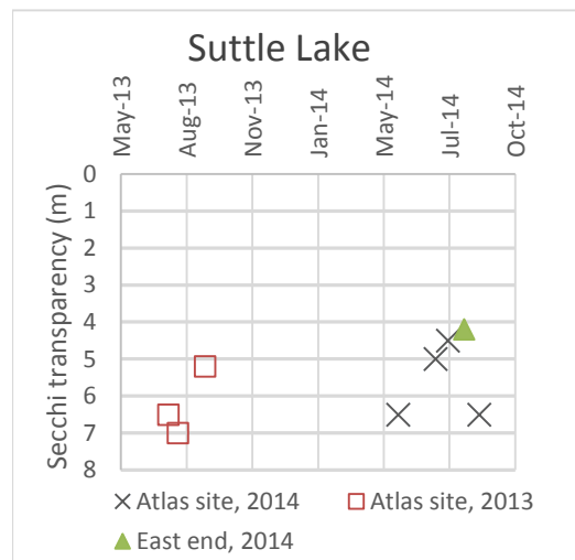
Figure 19. Suttle Lake location, temperature profile, and Secchi transparency.
