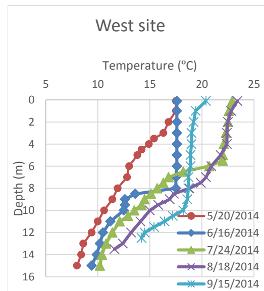
Figure 16. Prineville Reservoir location and temperature profiles.
