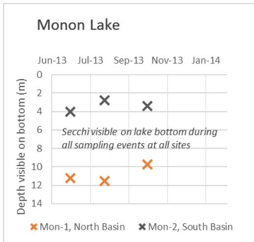
Figure 11. 2013 Monon Lake Secchi measurements.
