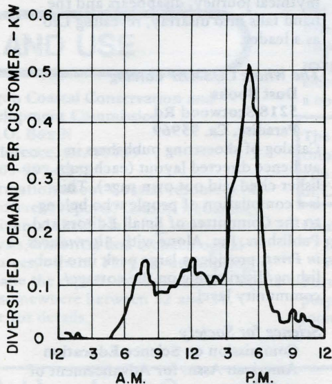
A daily load curve for an electric range. (Source: Federal Power Commission)
