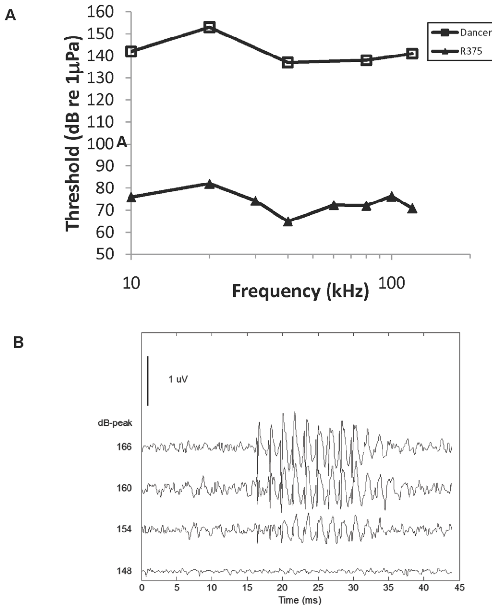
Figure 2. Results of hearing tests on two stranded rough-toothed dolphins. A. Audiogram of R375 (filled triangles), a normal hearing rough-toothed dolphin, and highest level tested for Dancer (open squares) rough-toothed (open squares) for which no response was detected at any frequency). For Dancer, there was at least a 70 dB hearing loss across all frequencies tested. B. Click-train (600 Hz click rate) evoked potential traces from the hearing-impaired rough-toothed dolphin (Dancer) at four stimulus levels. The click train sound starts at 15 ms. The lowest level detected was about 154 dB peak re 1 \mu Pa.
