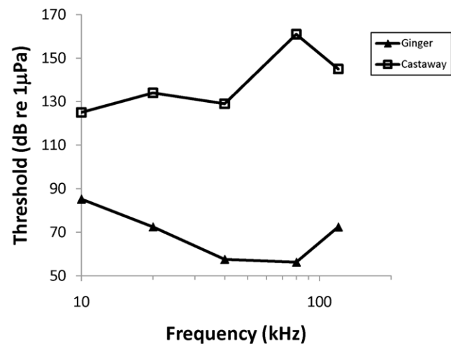
Figure 1. Audiogram of MML0807 (Ginger; filled triangles), a juvenile bottlenose dolphin with normal hearing, and MML FB303 (Castaway; open squares), an adult bottlenose dolphin with hearing loss. For Castaway, no response was detected at any frequency indicating that there was at least 40–100 dB hearing loss across all frequencies tested, and no response could be detected in response to click trains at 164 dB peak re 1 \mu Pa. doi:10.1371/journal.pone.0013824.g001
