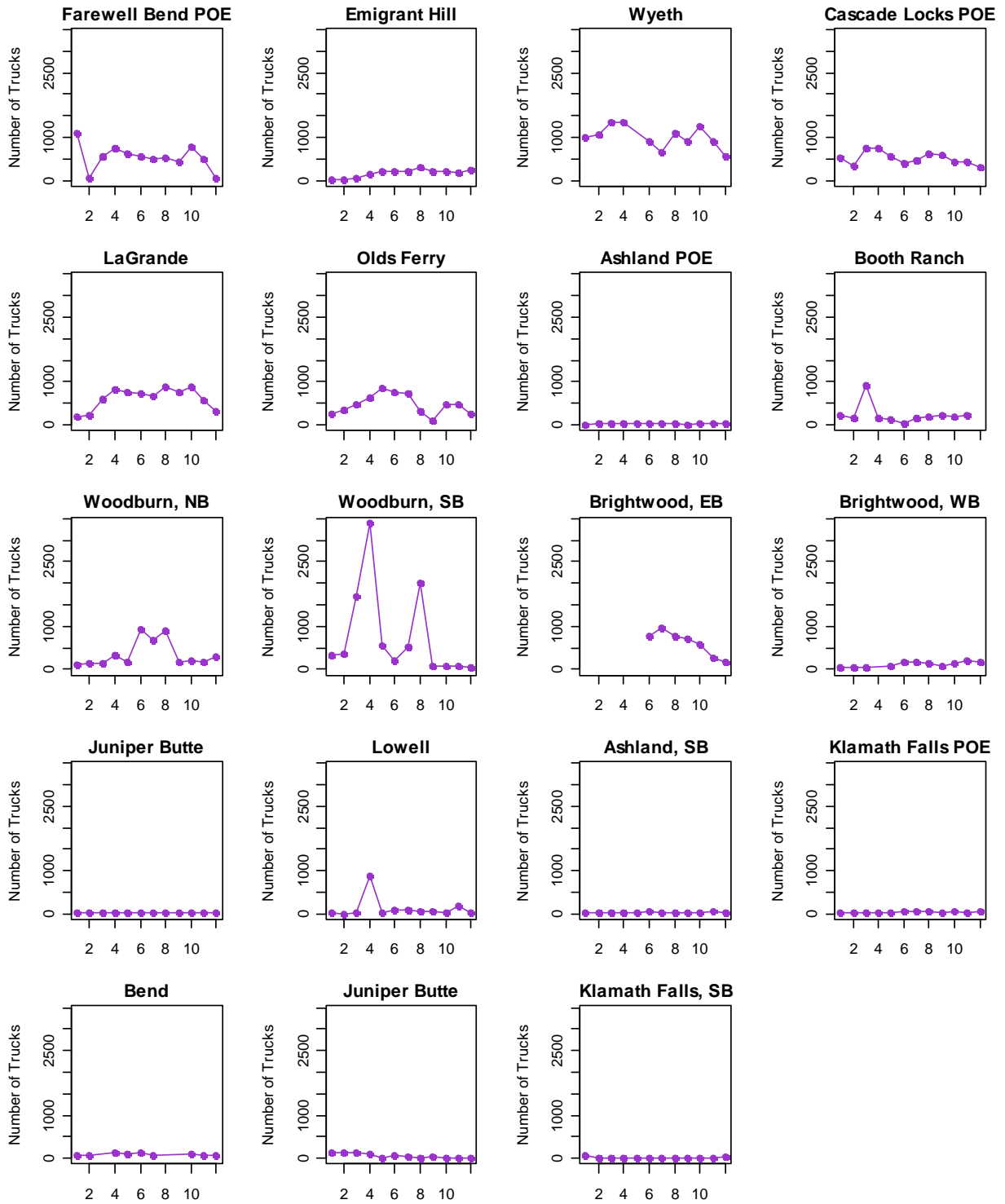
Figure 6.5: Number of Trucks Exceeding 105.5 kips by station, 2007
