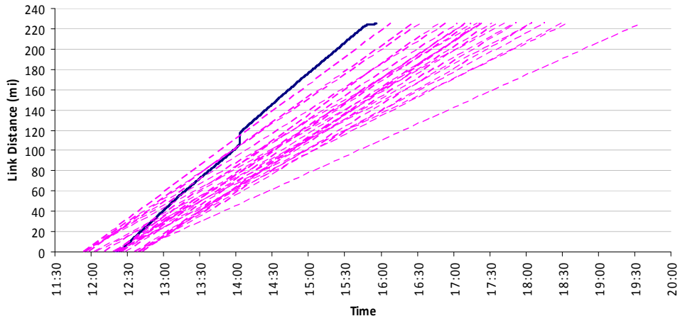
Modified Probe Path - Link_220 10_WDS to 16_ASS - Sep. 30
