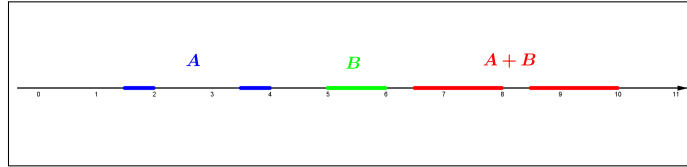
Figure 4.9: Set addition.
