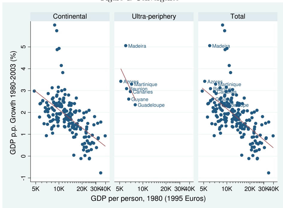
Figure 4: Convergence
