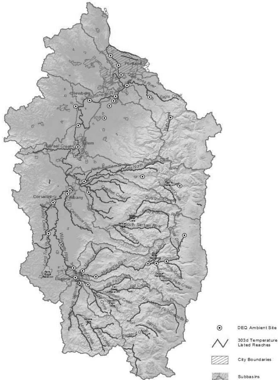
Figure 3-8. Willamette Basin map with temperature standard exceedances. Source: Oregon Department of Environmental Quality, 2006.
