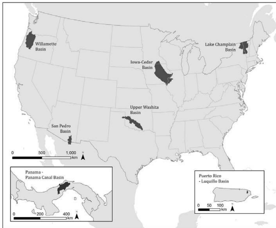
Figure 1. Locations of the UNESCO-HELP Basins in North and Central America.
