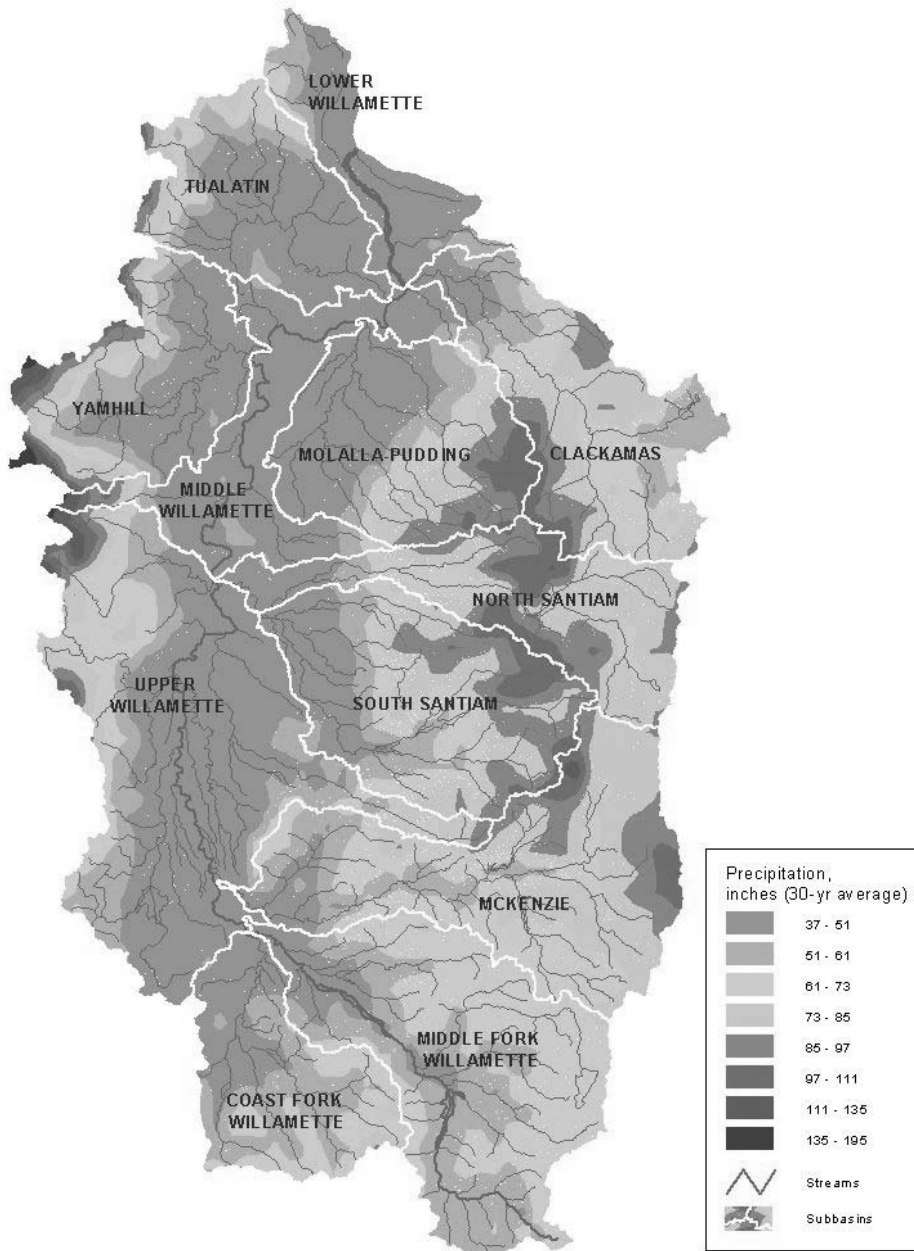
Figure 3-9. Spatial variations of mean annual precipitation in the Willamette Basin.
