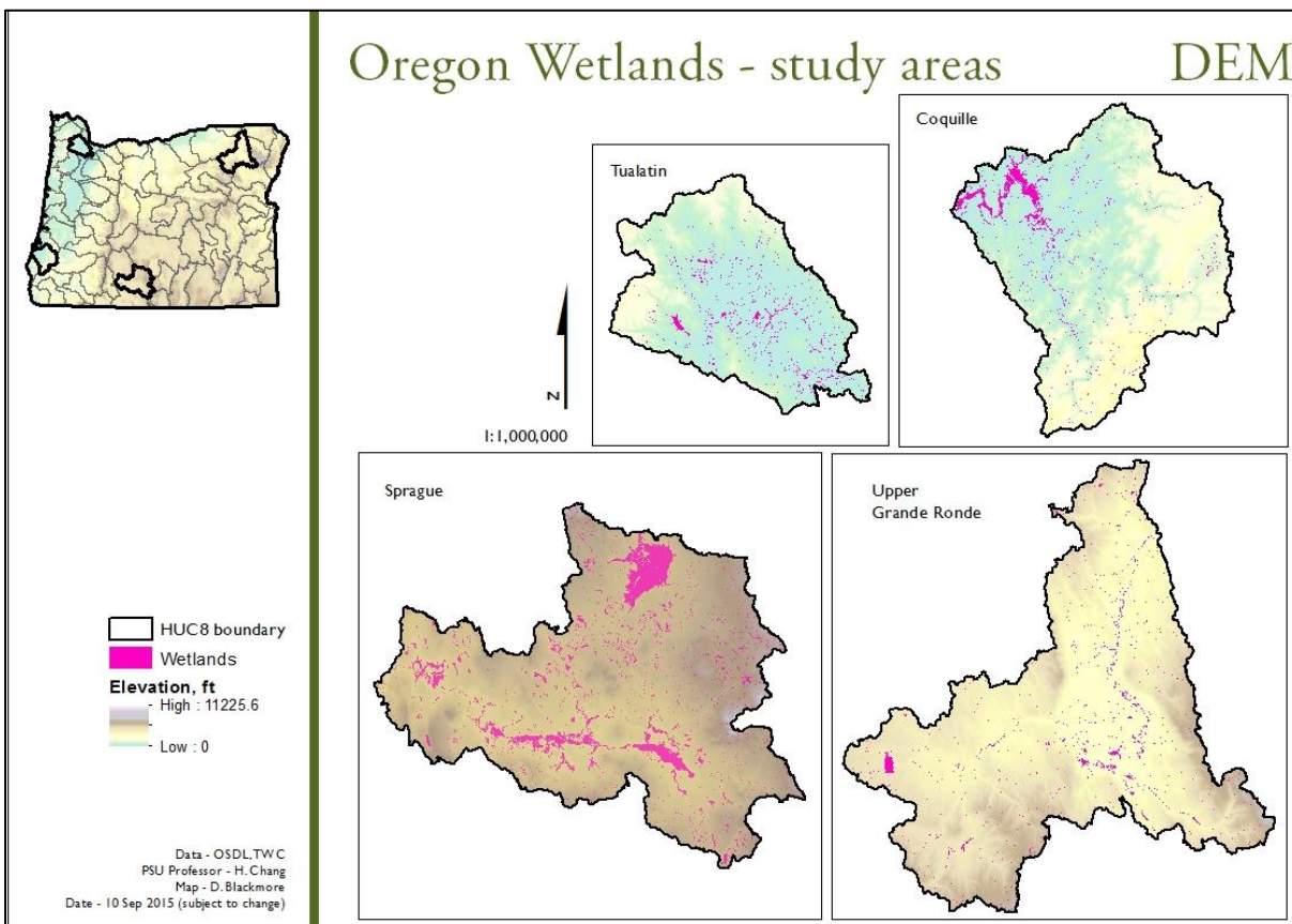
Figure 2. Study Areas. HUC8 subbasins in the State of Oregon with elevation, pilot study areas for the INR-PSU Wetland Prioritization Tool.
