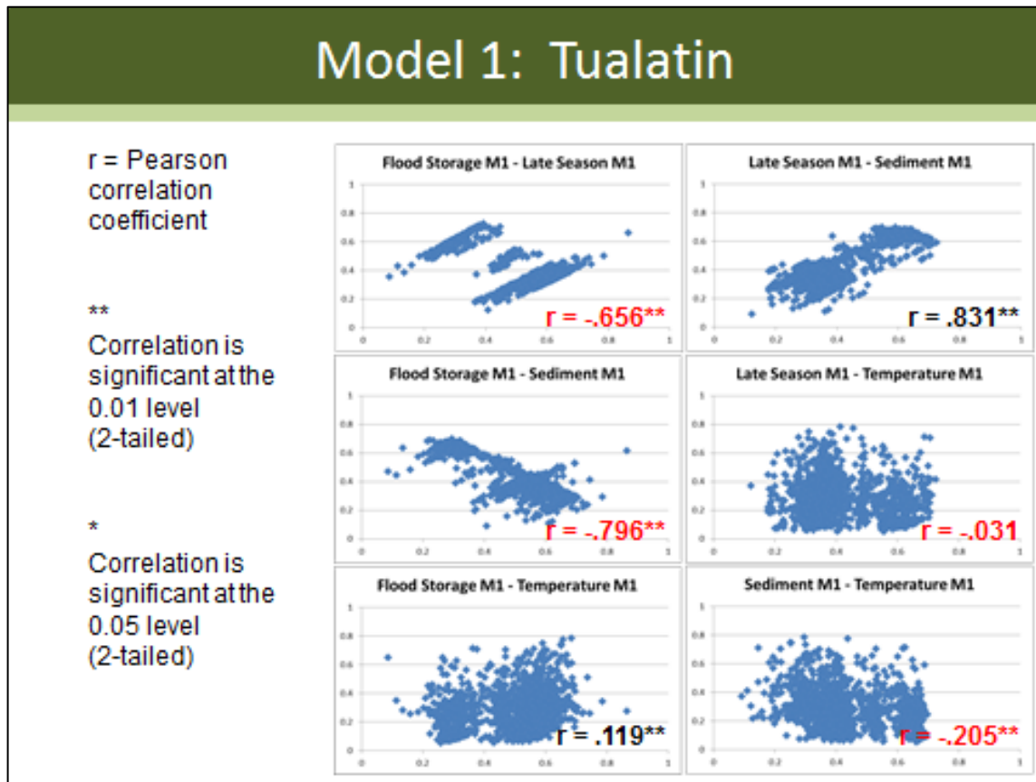
Figure 16. Correlations, Model 1, Tualatin. Bivariate correlations between estimates of wetland functions for Model 1 in the Wetland Prioritization Tool.
