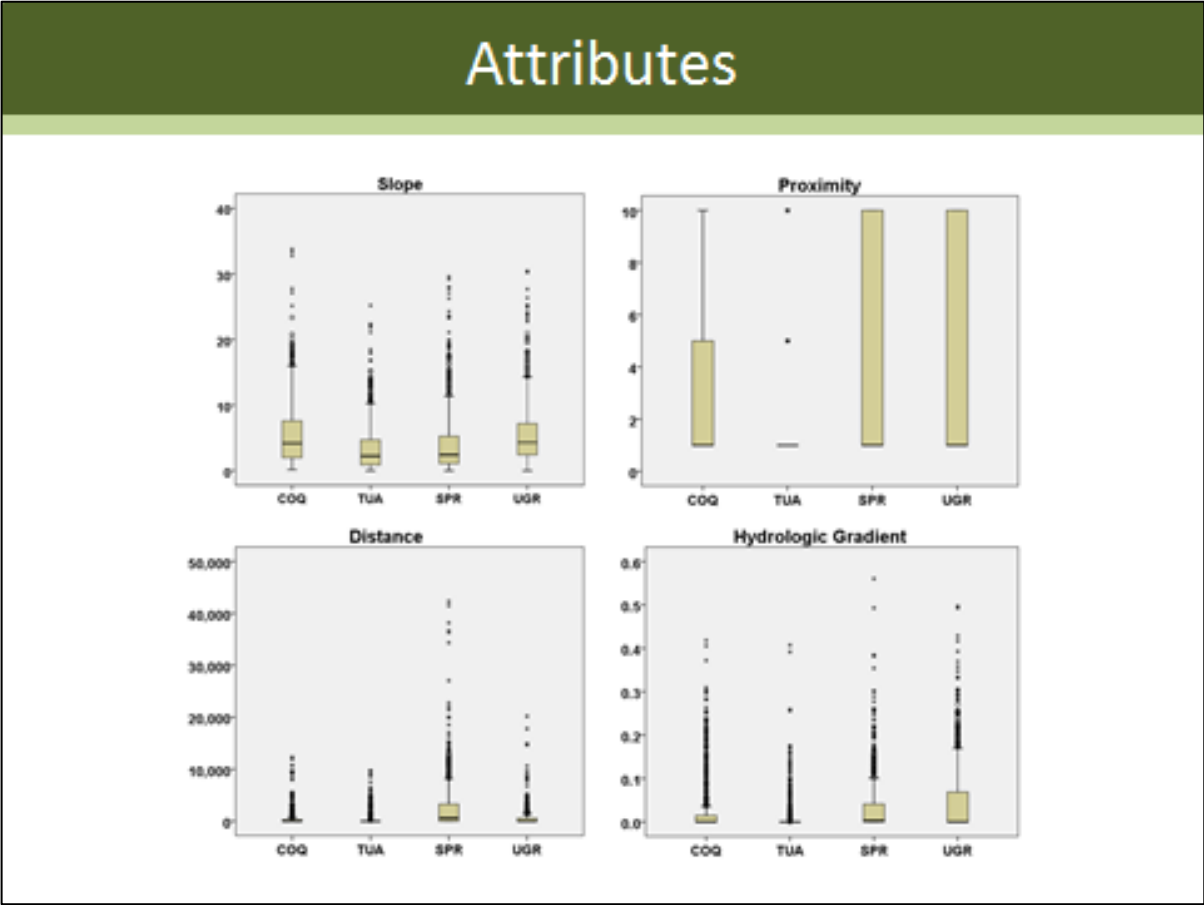
Figure 29. Boxplots, Attributes 2 of 3. Box and whisker diagrams showing distribution of selected attribute values across study areas for the Wetland Prioritization Tool.
