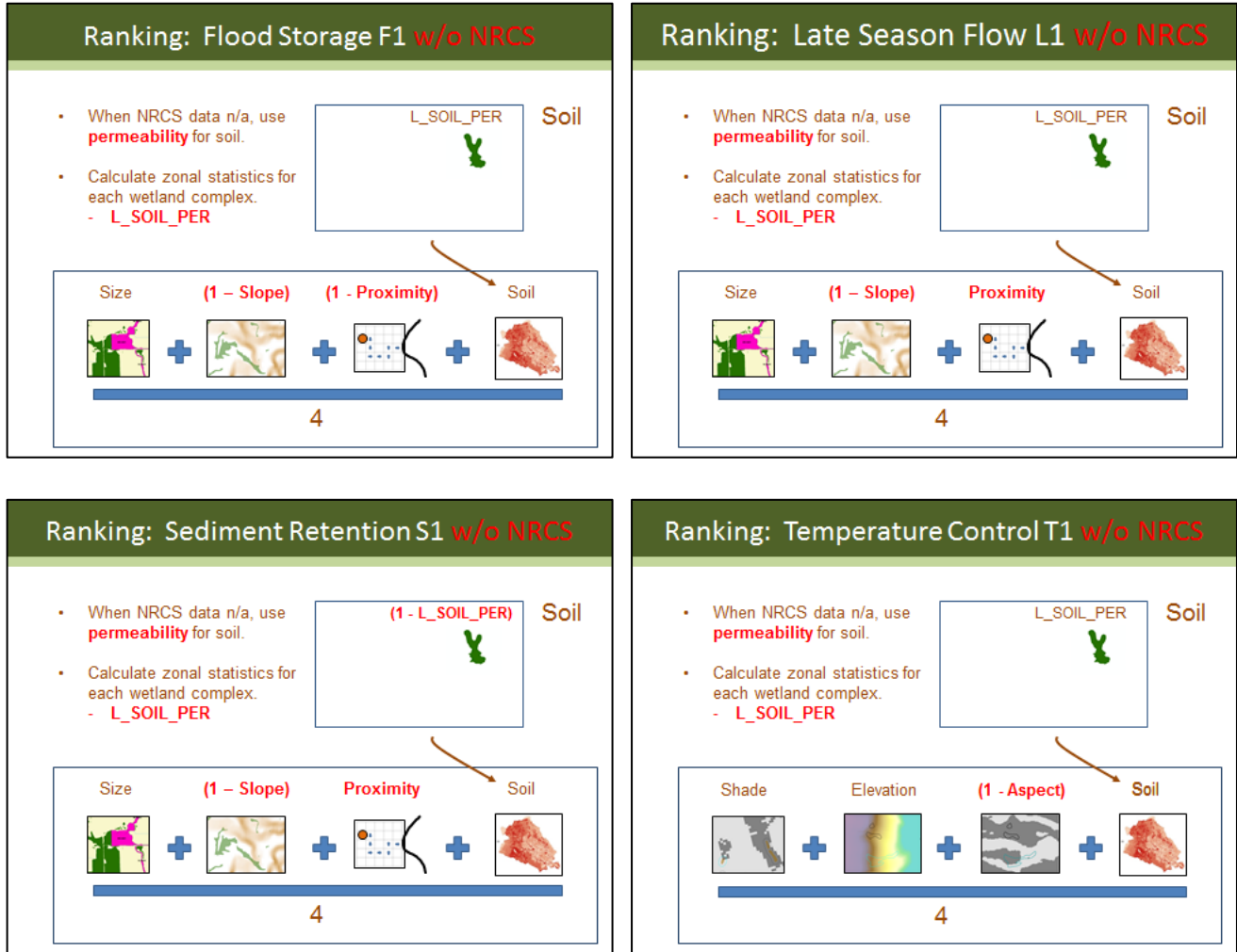
Figure 13. Equations for non-NRCS. Visual depictions of wetland function calculations in the INR-PSU Wetland Prioritization Tool, highlighting the exchange of soil permeability data in areas where NRCS soil survey data is unavailable. Similar substitutions can be made for Model 2.
