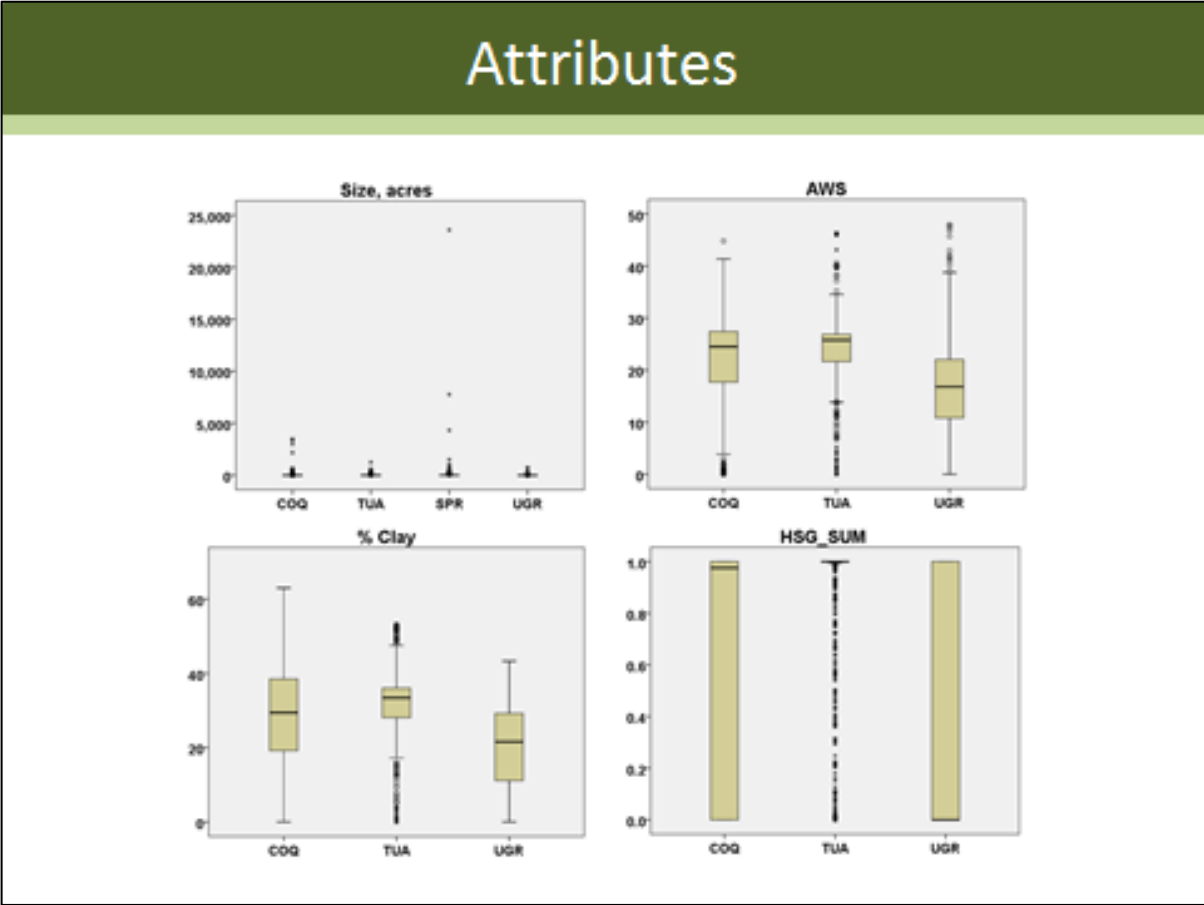
Figure 28. Boxplots, Attributes 1 of 3. Box and whisker diagrams showing distribution of selected attribute values across study areas for the Wetland Prioritization Tool.
