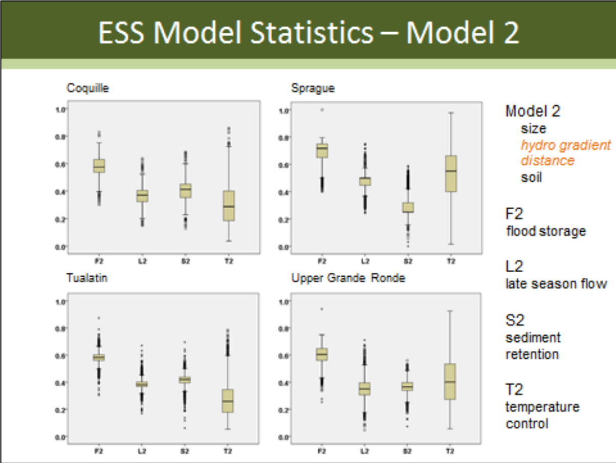
Figure 27. Boxplots, Model 2. Box and whisker diagrams showing distribution of Model 2 estimates for wetland functions.
