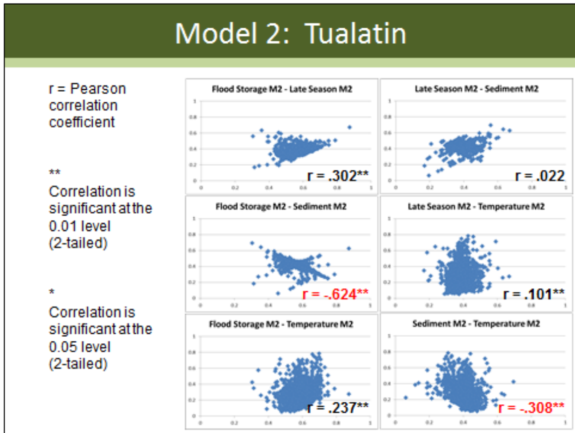
Figure 20. Correlations, Model 2, Tualatin. Bivariate correlations between estimates of wetland functions for Model 2 in the Wetland Prioritization Tool.
