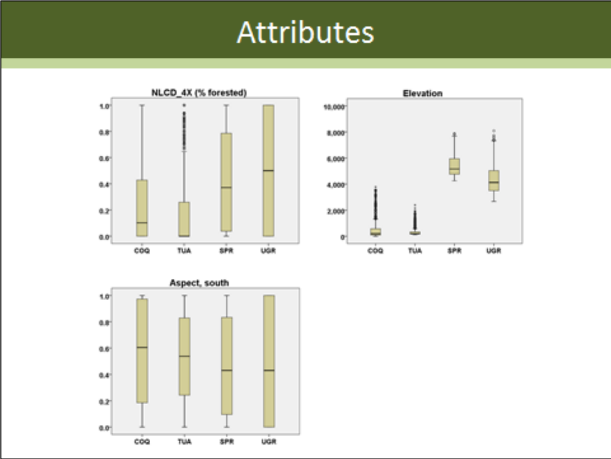
Figure 30. Boxplots, Attributes 3 of 3. Box and whisker diagrams showing distribution of selected attribute values across study areas for the Wetland Prioritization Tool.
