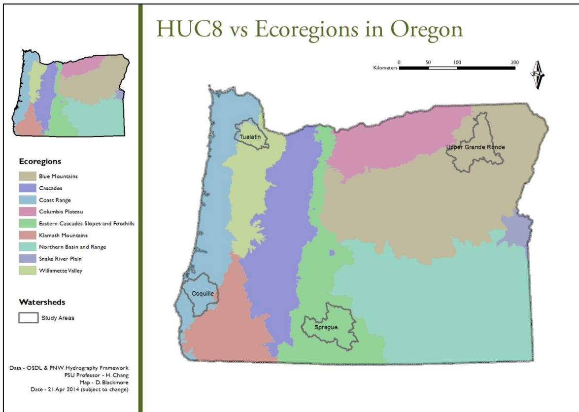
Figure 1. Ecoregions. Level III ecoregions in the State of Oregon showing study areas for the INR-PSU Wetland Prioritization Tool, including subbasins Coquille, Sprague, Tualatin & Upper Grande Ronde.
