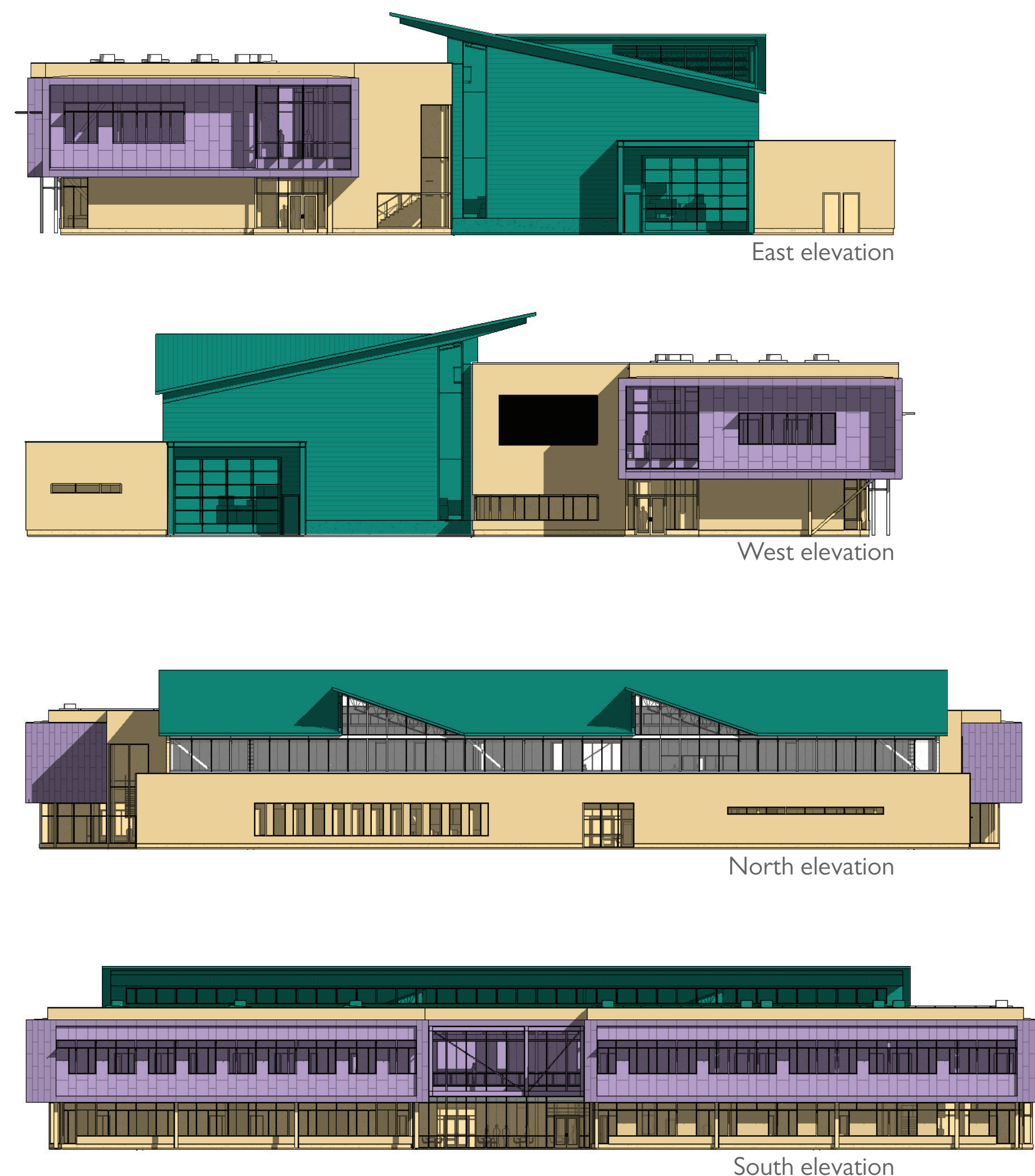
Yellow Box rib metal panel vs brick vs CMU Purple Dri-Design metal panel (to remain) Teal Kingspan IMP vs MP w/ insulation
