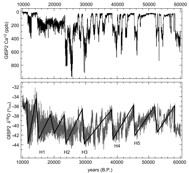
Figure 6. The Ca +2 and the δ 18 O records from the GISP2 ice core (upper panel and lower panel, respectively). Data are adapted from Mayewski et al. [1997] and Stuiver and Grootes [2000] using the GISP2 timescale [Meese et al. , 1997]. Superimposed on the δ 18 O record (heavy black line) is the qualitative pattern of change referred to as the Bond cycle [Bond et al. , 1993]. The placement of the Heinrich events, labeled H1-H5, in the lower panel follows Bond et al. [1993]. Note that H2 and H3 are accompanied by particularly strong Ca +2 spikes. Cooling events between H4 and H3 and between H3 and H2, some coeval with pronounced Ca +2 spikes, are not accompanied by ice-rafted debris pulses from the LIS.
