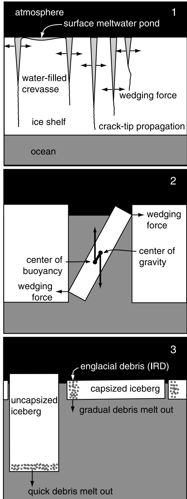
Figure 2. Ice shelf cross sections depicting processes associated with sudden ice shelf disintegration. Climate warming initiates the process via surface meltwater (panel 1). Water-filled crevasses propagate downward to the ice shelf bottom, eventually allowing discrete, independent ice shelf fragments to develop. Some fragments will begin to capsize spontaneously, converting buoyancy-driven capsize torque into forces that push apart the surrounding ice shelf apart (surrounding ice depicted for simplicity as unfractured, panel 2). Approximately 50% of the original, prebreakup area of Larsen B Ice Shelf, for example, broke into icebergs that subsequently capsized by rolling 90° onto their sides (panel 3). Gravitational potential energy released by capsize drives the final stages of the ice shelf's explosive disintegration, and yields icebergs with debris bands (as shown in panel 3) that are favorably oriented for long-term survival in transatlantic drift.
