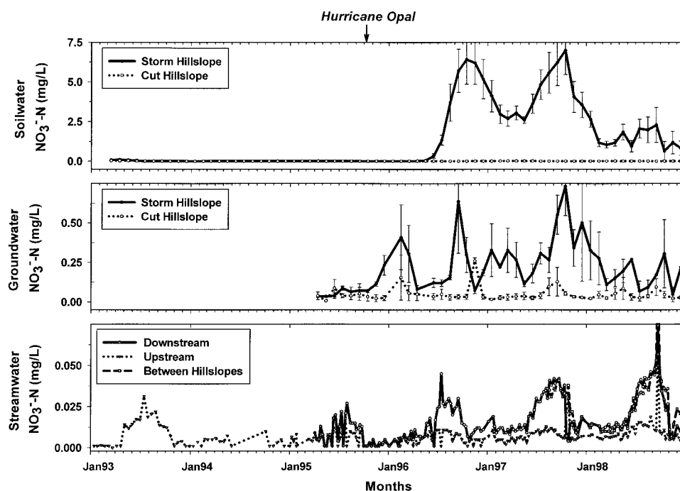
Figure 8. Mean \text{NO}_3^- -N concentrations in soilwater, groundwater, and streamwater over the period of the study. Soilwater samples were taken from the B horizon lysimeters in the area 0–5 m from stream. Groundwater samples were taken from piezometers located at the lowest lysimeter site on each hillslope. Streamwater samples upstream were taken from the WS 56 weir from January 1993 to March 1995, and then from above both hillslopes from April 1995 to December 1998. Streamwater samples downstream of the hillslopes were taken from April 1995 to December 1998. Streamwater samples between hillslopes were taken from August 1997 to December 1998.
