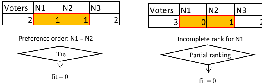
Figure 2a and 2b: tie, and partial ranking examples
