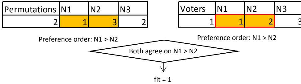
Figure 1a: preference order fit example
