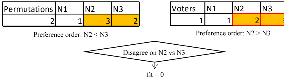
Figure 1b: preference order does not fit example
