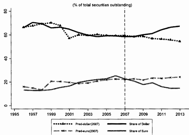
(a) Full Sample – Counterfactual
