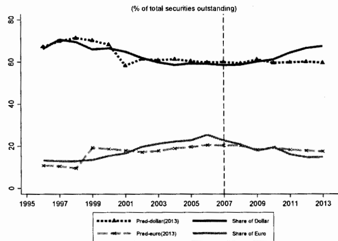
(c) Full Sample with in-sample prediction
