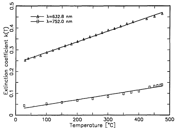
Fig. 4. Extinction coefficient as a function of temperature for the \alpha -Si sample.
