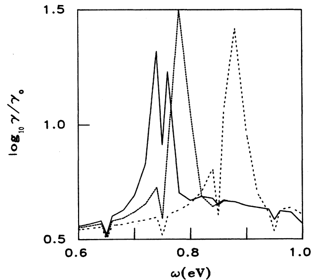
FIG. 9. Cross coupling into the long- and short-range surface plasmons for the configuration as in Fig. 8 for thinner film thicknesses ( t = 150 Å). Only the cases b (dashed line), d (dotted line), and e (solid line) of Fig. 8 are shown.
