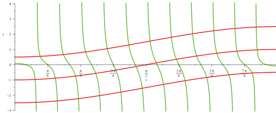
FIG. 3.1. The three cases of Proposition 3.5. The fast varying (green) plot is the left-hand side of (3.2), and the slow varying (red) curves represent its right-hand side in cases 1, 2, and 3 (from top to bottom).
