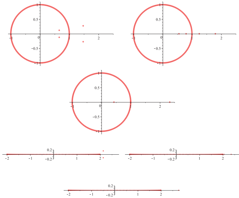
FIG. 4.1. Numerical illustration of the roots of P(y) (top) and the eigenvalues (bottom) for three different parameter values (given in text)
