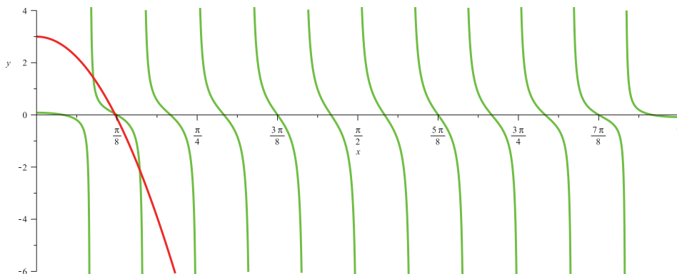
FIG. 3.3. Detail of case 2b of Proposition 3.7: a = 1 , e = -1.05 , and dr = -1.9 . Here n = 12 . The multiple roots in the second branch disappear for large n (while holding other parameters fixed).
