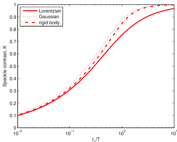
Fig. 5. (Color online) Speckle contrast as a function of integration time for various intensity correlation laws.
