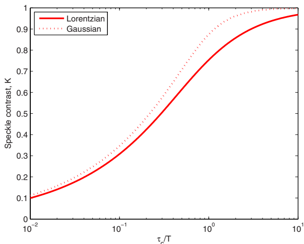
Fig. 2. (Color online) Speckle contrast as a function of relative integration time for Lorentzian and Gaussian autocorrelation functions.
