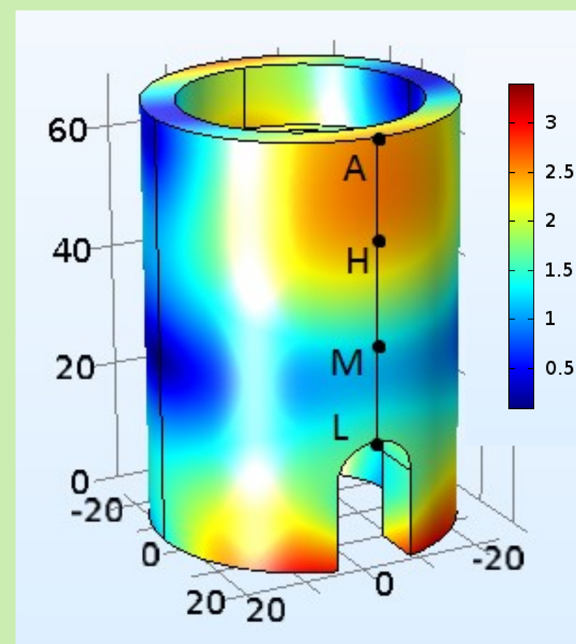
Fig.4 Mapping of a particular acoustic mode w/2\pi = 28 \text{ kHz}
