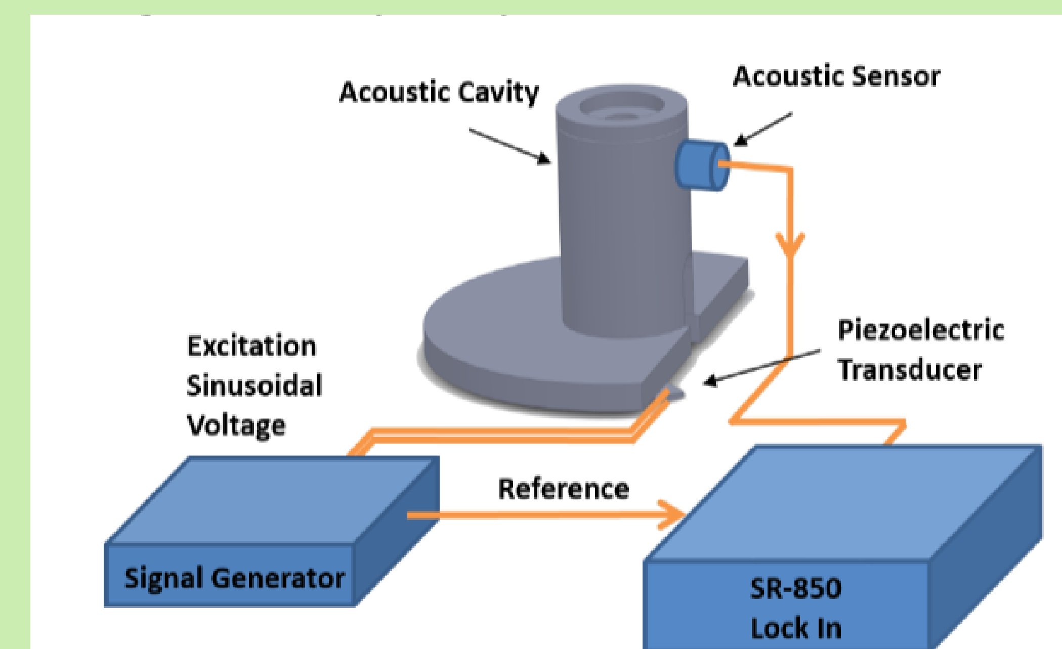
Fig.3 Experimental Setup:
