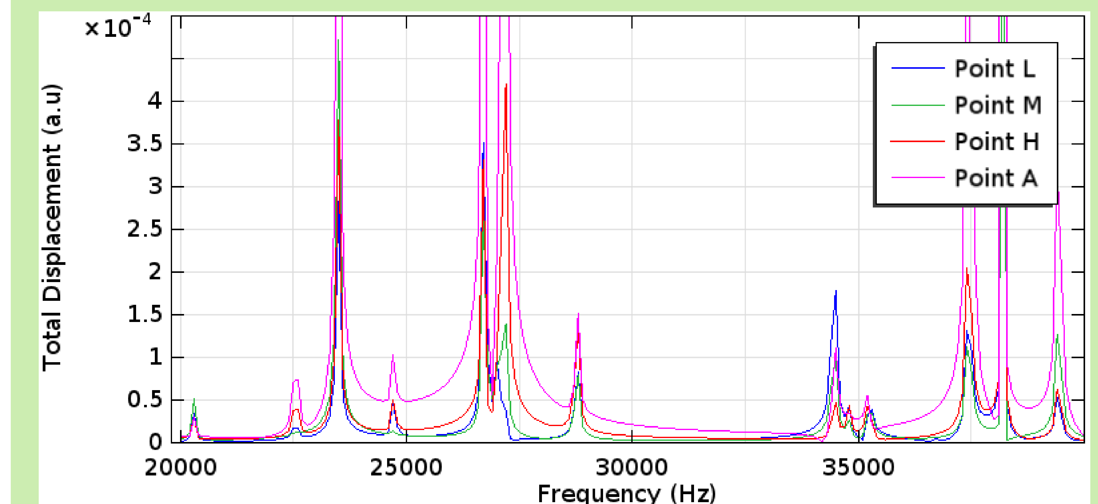
Fig. 5 Frequency Response: Total displacement of the acoustic mode at different locations of the cavity vs frequency.
