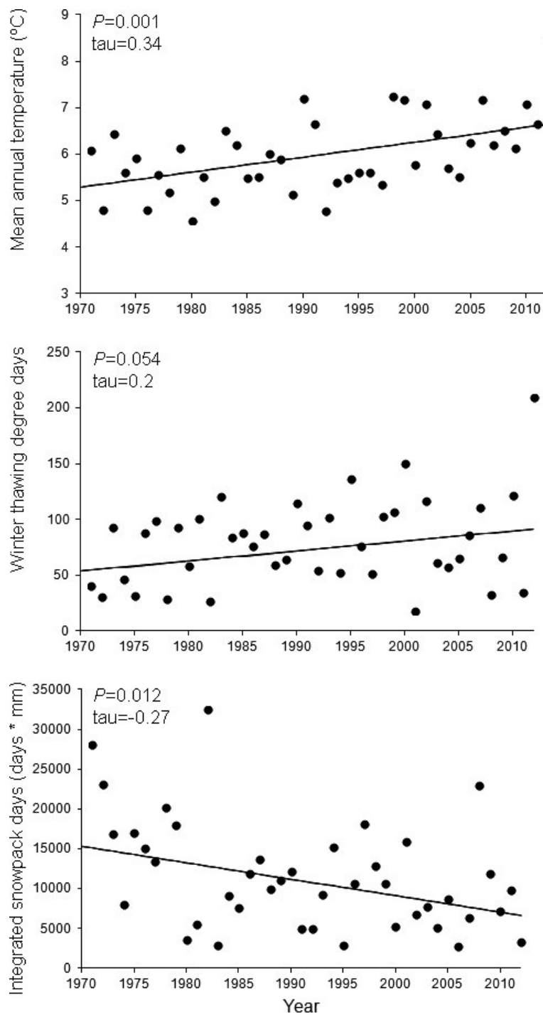
Fig. 5. Mann-Kendall analyses and Sen slopes for the long-term records of mean annual air temperature (490 m), winter thawing degree days (490 m), and integrated snowpack days (560 m) at the Hubbard Brook Experimental Forest, New Hampshire, USA.
