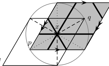
Figure 2.4b: A Type II space
