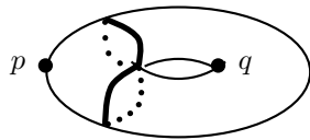
Figure 2.4a: A Type I space
