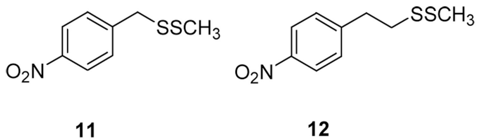
Figure 3. p -Nitrobenzyl and p -nitrophenethyl disulfides 11 and 12 .
