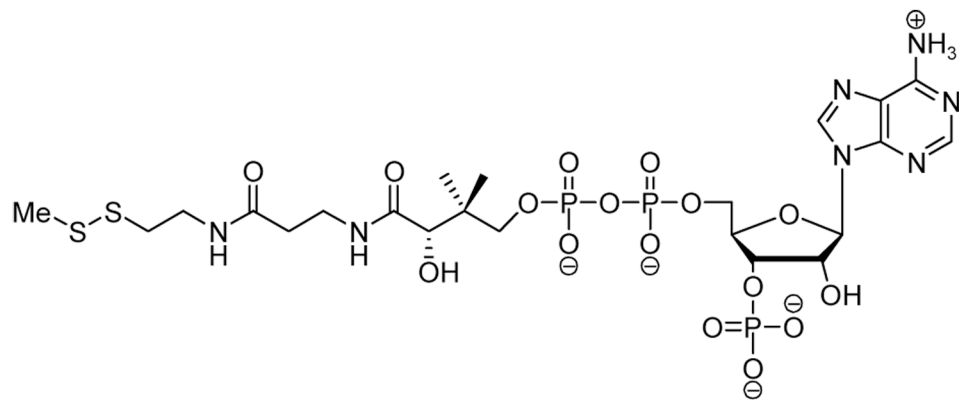
Figure 6. Methyl-coenzyme A mixed disulfide.
