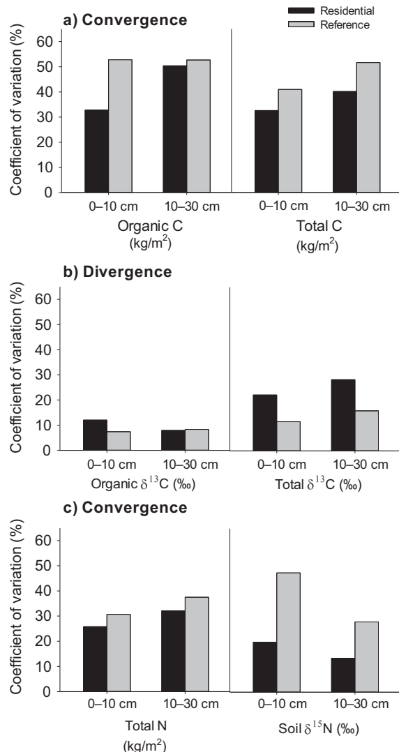
FIG. 1. Coefficient of variation (%) across the six cities exhibits convergence for (a) soil organic and total soil C ( \text{kg}/\text{m}^2 ) and for (c) soil total N ( \text{kg}/\text{m}^2 ) and \delta^{15}\text{N} (‰), yet exhibits divergence for (b) soil organic and total \delta^{13}\text{C} (‰) in residential yards compared to reference sites.
