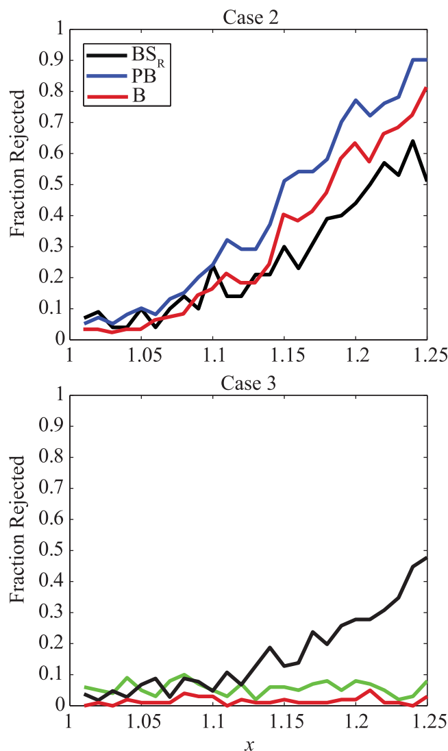
Figure 5. Fraction of forecasts rejected via the reliability component of the Brier Score ( BS_R ), the Poisson-Binomial distribution (PB), and the Binomial distribution (B), from 100 replicates, for varying x values (equation (18)) of case 2 and 3.
