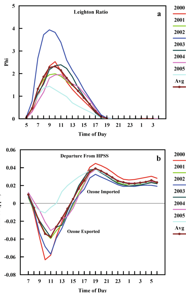
Fig. 5 a The Leighton ratio, b \delta(O_3) representing the departure of the observed ozone from a hypothetical photo-stationary state. The departure of the Leighton ratio from 1 is driven by the presence of peroxy radicals generated from the oxidation of the VOCs and by transport process that carry ozone and its pre-cursors to and from the location of the measurements
