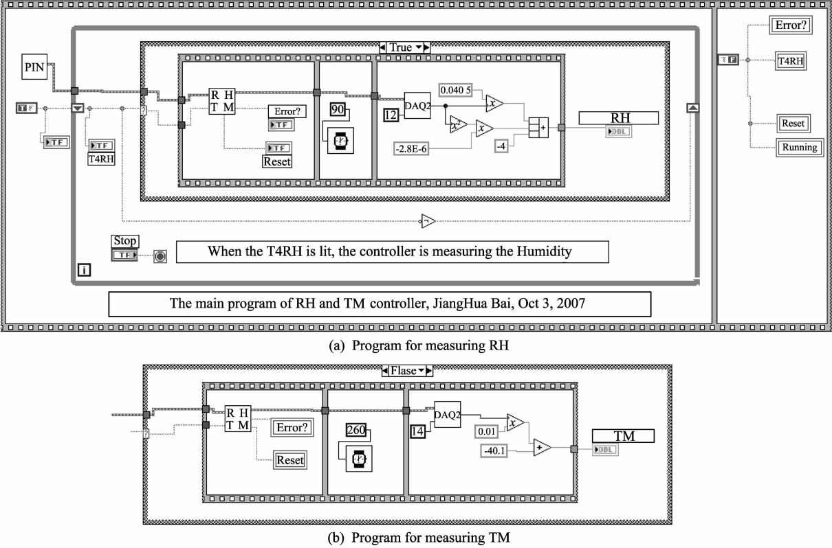
Fig. 5 Main program of SHT75 driver
