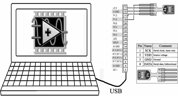
Fig. 2 A simple illustration of hardware connection
