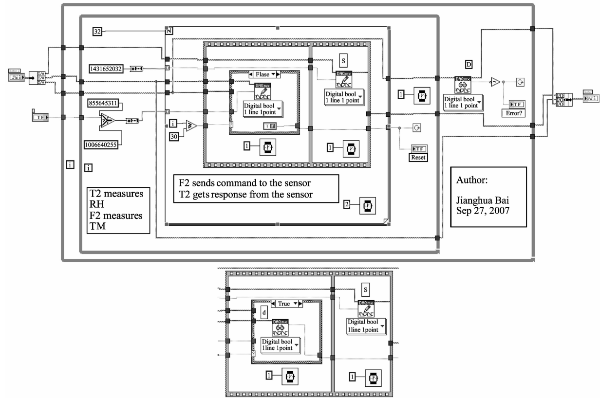
Fig. 8 RH-TM subroutine
