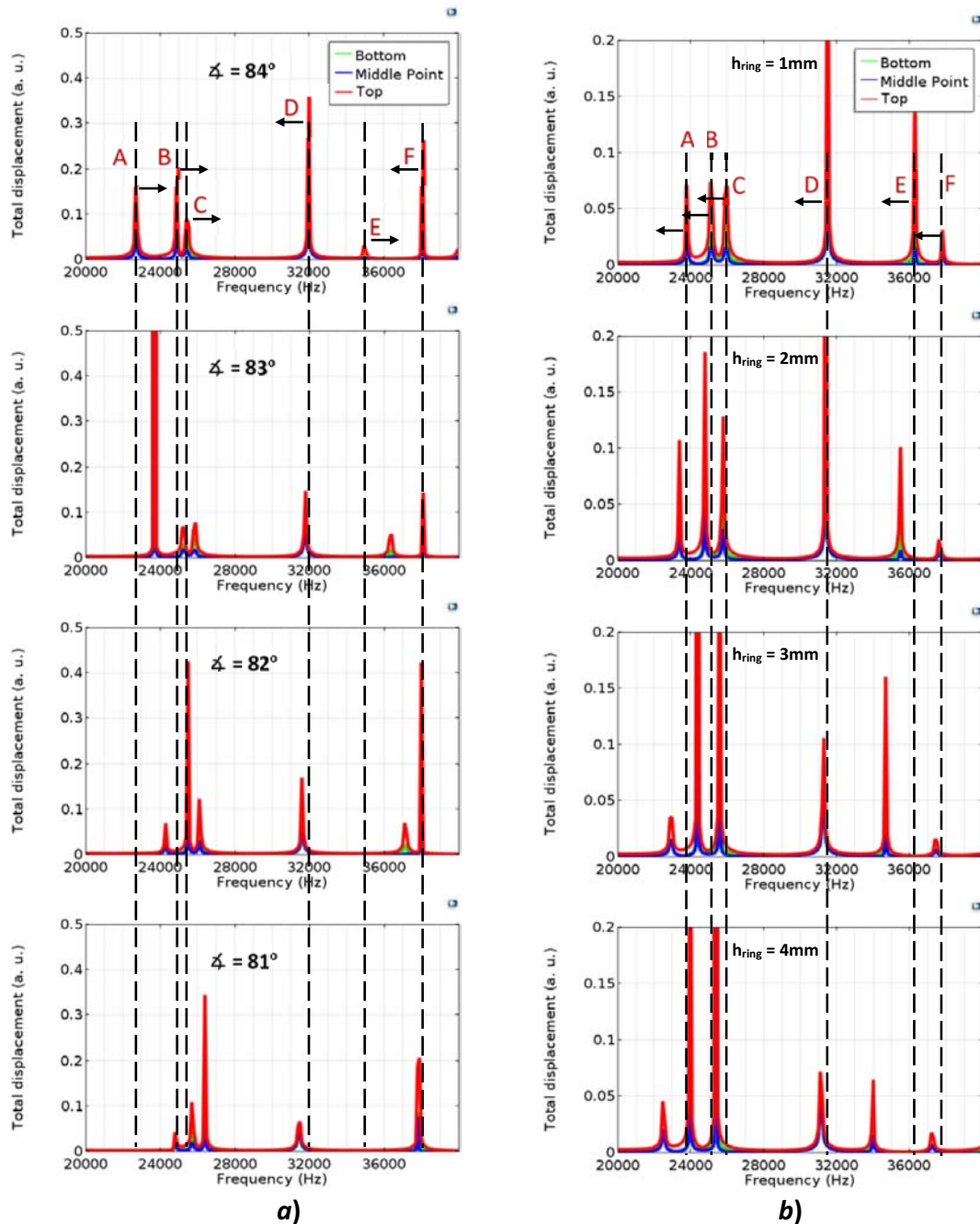
Figure 7. Spectral response variations as a) the cone angle of the cavity increases, and b) when adding rings of different thicknesses ( h_{\text{ring}} in Fig. 4) to the top of the cavity.
