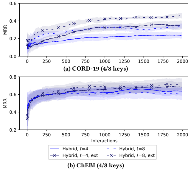
Figure 6: External feature comparison (Zipf, 4/8 keys)
