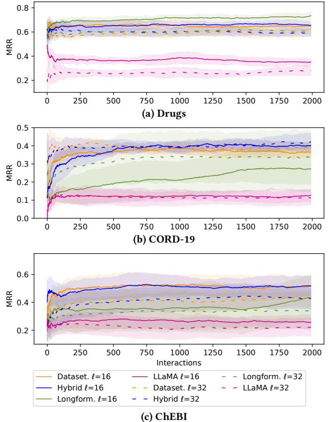
Figure 5: Dataset, Hybrid, and LM-based (Zipf, 16/32 keys)
