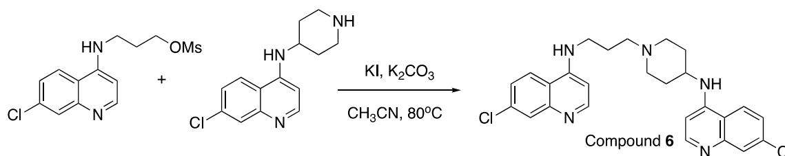
Figure 12. Synthesis of Compound 6.
