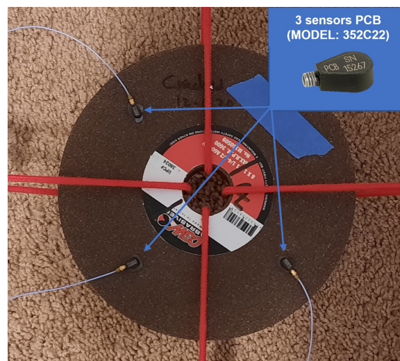
Figure 5. Measurement setup for impact hammer testing.
