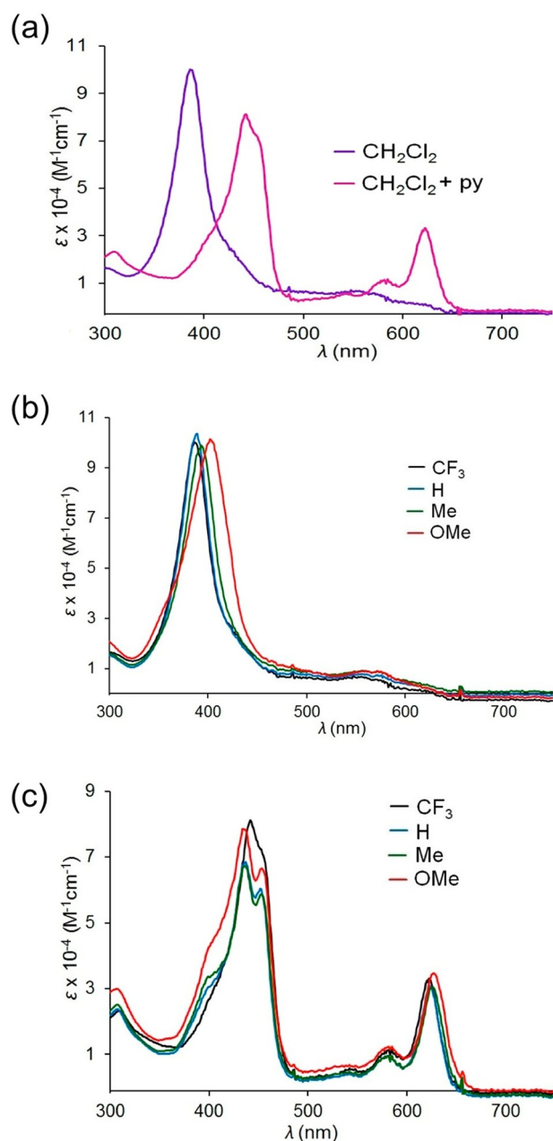
Figure 19. UV–vis spectra of (a) \text{Co}[\text{TpCF}_3\text{PC}](\text{py})_2 , (b) the \text{Co}[\text{TpXPC}](\text{py})_2 series in \text{CH}_2\text{Cl}_2 , and (c) the \text{Co}[\text{TpXPC}](\text{py})_2 series in \text{CH}_2\text{Cl}_2 with 0.5% pyridine. Reproduced from ref 68. Copyright 2017 American Chemical Society.
