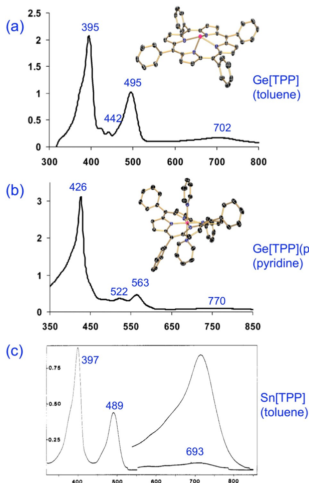
Figure 2. UV-vis-NIR spectra of reduced Ge and Sn porphyrins. Adapted with permission from refs 15 and 16. Copyright 2007 and 1990, respectively, American Chemical Society.
