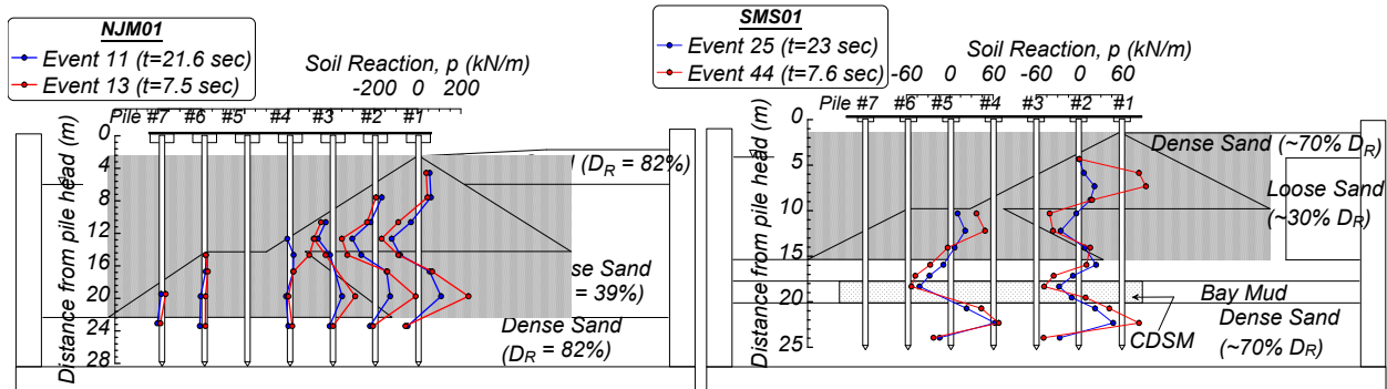
Fig. 6. Soil reaction profiles at the time of maximum bending moment in NJM01 and SMS01.
