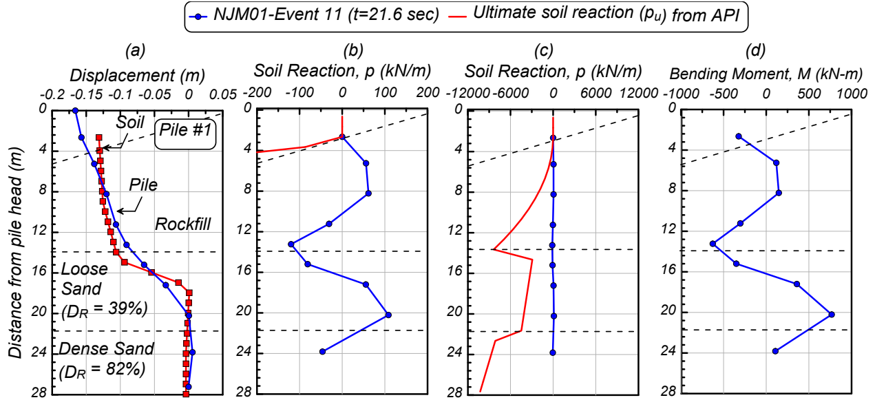
Fig. 7. (a) Displacement, (b) soil reaction at small scale, (c) soil reaction at large scale, and (d) bending moment profiles at the time of maximum bending moment for Pile 1 in NJM01 Event 11.
