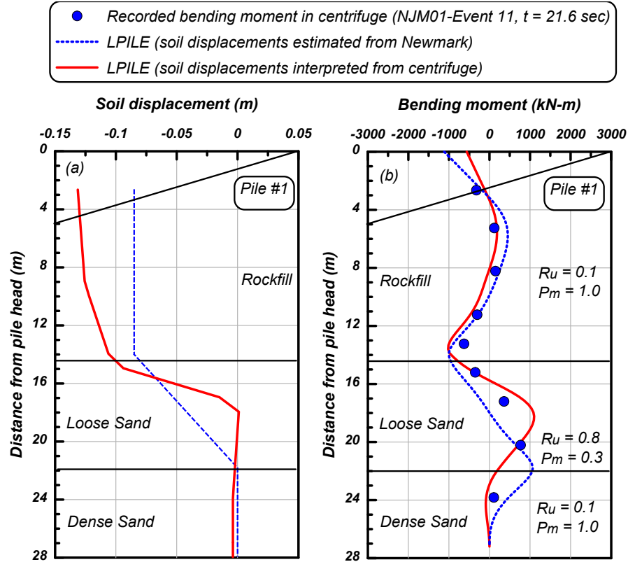
Fig. 5. (a) Comparison of soil displacement profiles interpreted from centrifuge test (peak transient) and estimated in design (mean Newmark) for Pile #1 in NJM01. (b) comparison of estimated bending moments from LPILE and measured bending moments from centrifuge
