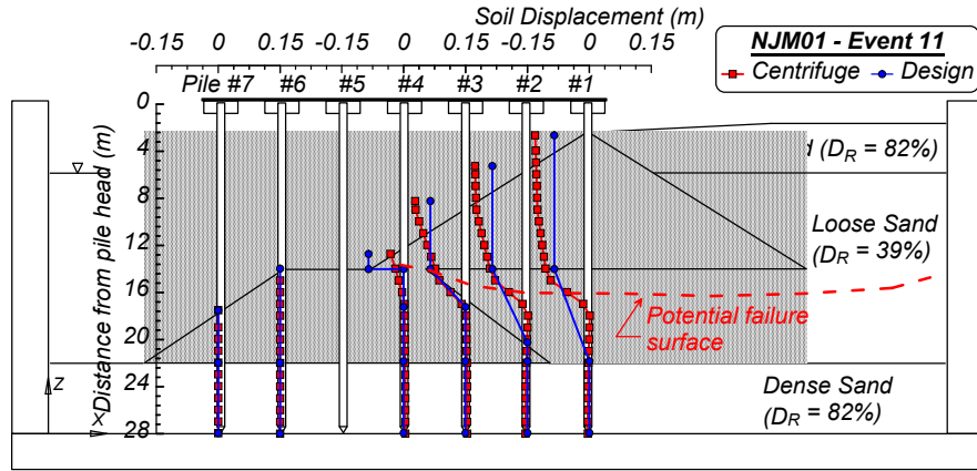
Fig. 3. Comparison of soil displacements at pile locations estimated in design (mean Newmark) and interpreted from centrifuge test results (peak transient) for NJM01 Event 11.
