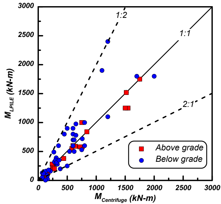
Fig. 9. Comparison of maximum bending moments recorded from centrifuge and predicted from LPILE baseline analyses (soil displacements and pile head shear extracted from centrifuge) for all five centrifuge tests
