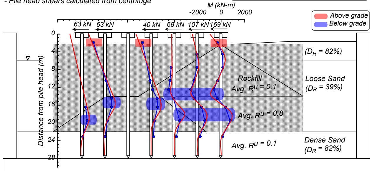
Fig. 8. Comparison of recorded maximum bending moments for all instrumented piles in NJM01 Event 11 with estimated values from the baseline analysis in LPILE
