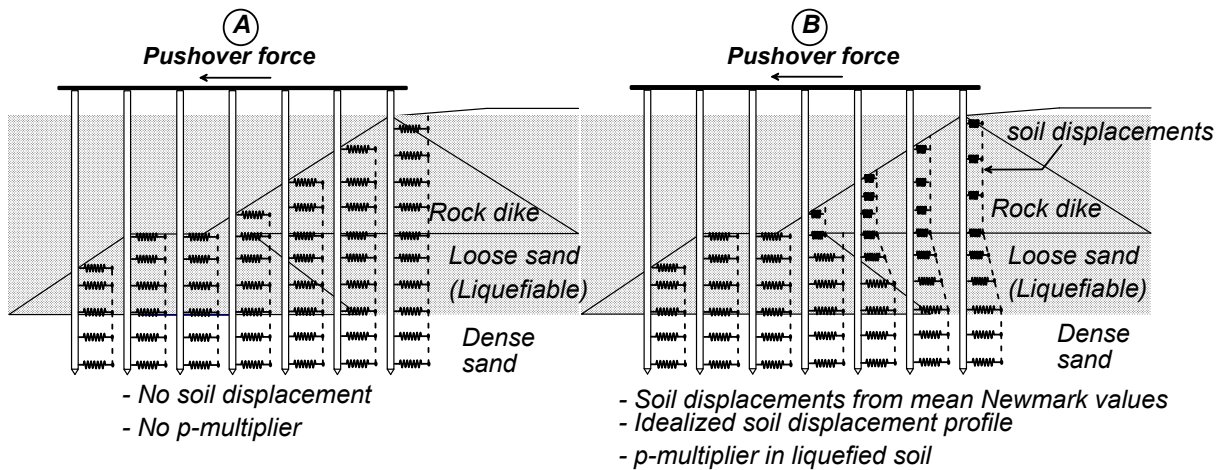
Fig. 10. Schematic of (a) nonliquefied and (b) liquefied pushover analyses.
