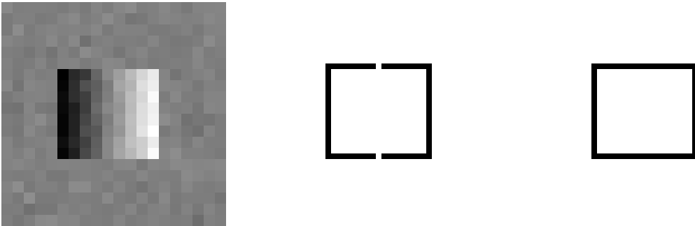
Figure 5.2. Ramp image from Leclerc's paper [48] (left), C^0 -discontinuities in reconstruction with difference terms from Section 2.4 (middle), and C^0 -discontinuities with revised difference terms from Section 5.2 (right).
