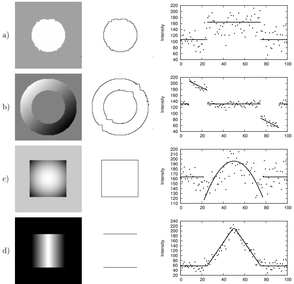
Figure 4.7. Results with test-case specific parameter values: a) b = 0.31, d = 0.96 , b) b = 0.26, d = 0.16 , c) b = 0.41, d = 0.01 , d) b = 0.66, d = 0.31 . The display above is similar to Figure 4.5, but the center column shows the C^0 -discontinuities in the reconstruction.
