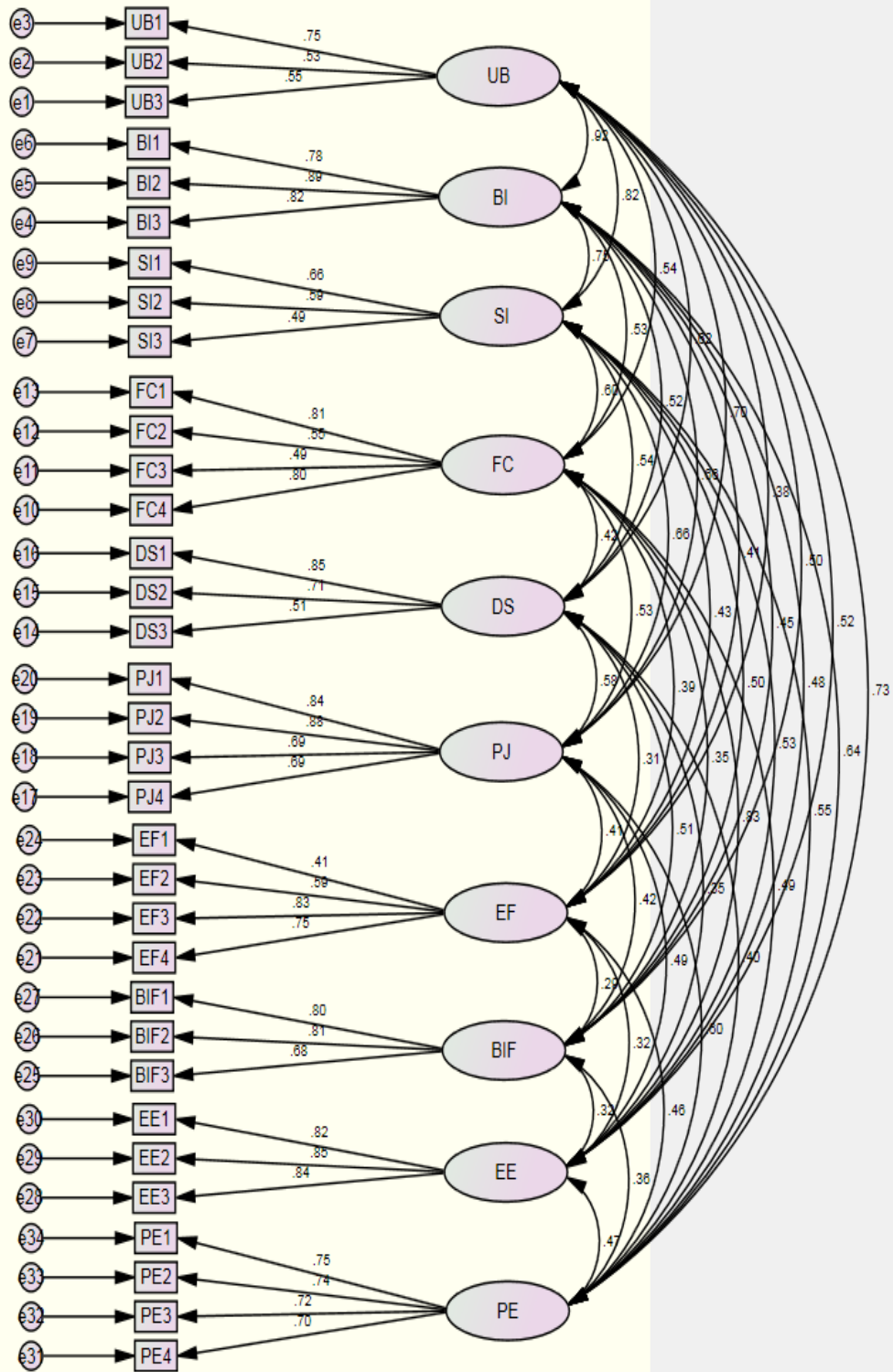
Figure 14: Measurement Model
