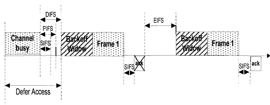
Figure 11: Frame retransmissions due to ACK failure
