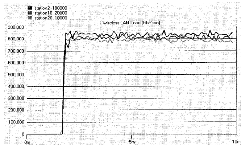
Figure 15: The global traffic loads
