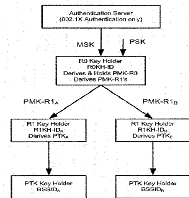
Figure 32: The new key hierarchy
