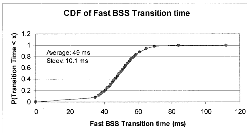
Figure 36: CDF of BSS Transition Optimization Time
