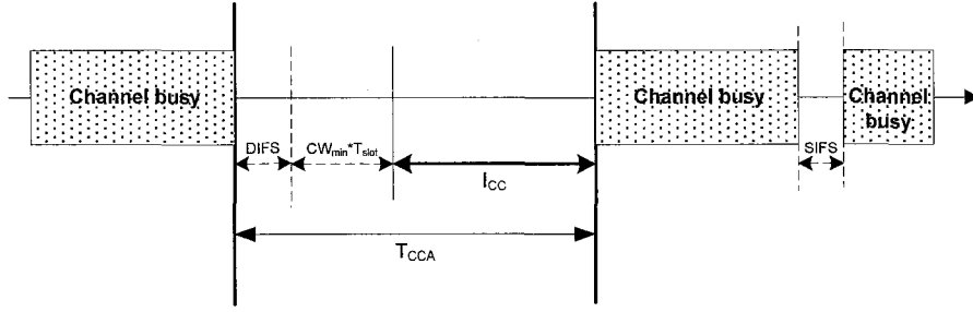
Figure 20: Clear channel time measurement
