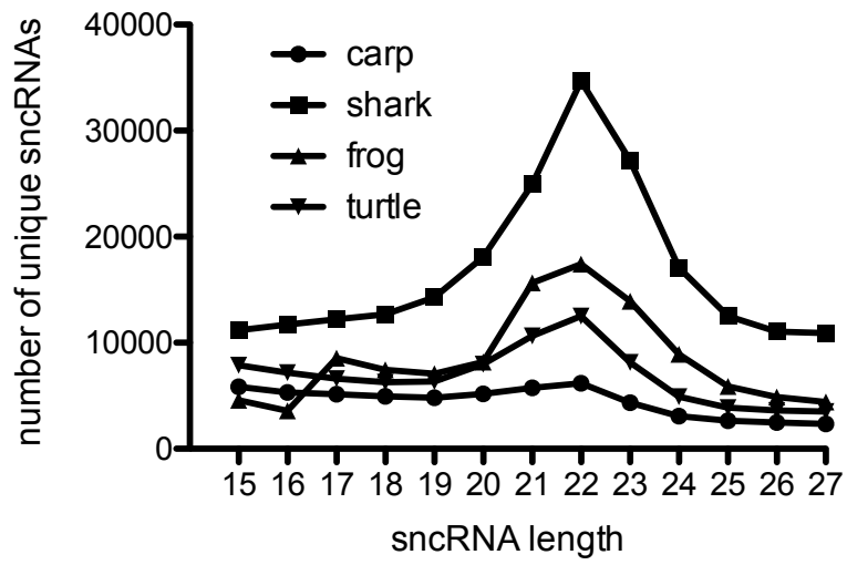
Figure S2. Length distribution of unique small RNAs identified in each species.
