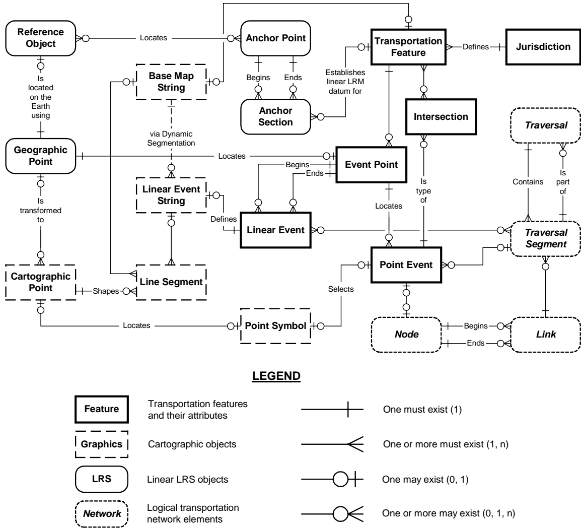
Figure 1. Simplified Enterprise GIS-T data model.
